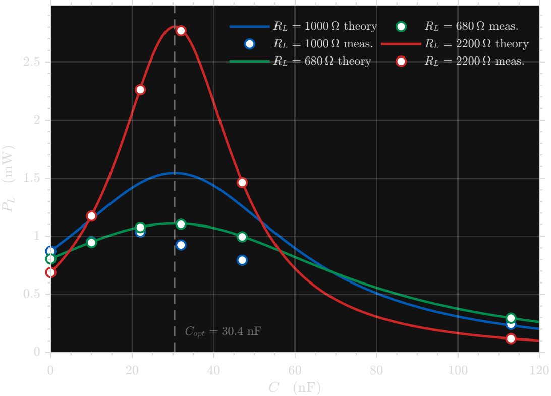
Case 2: load power vs. shunt capacitance
